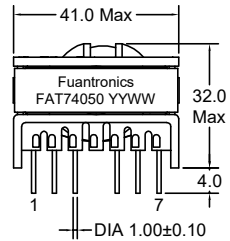
Orthographic view
